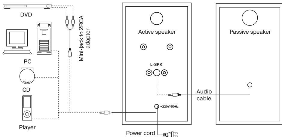
Fig. 2. Connection diagram
